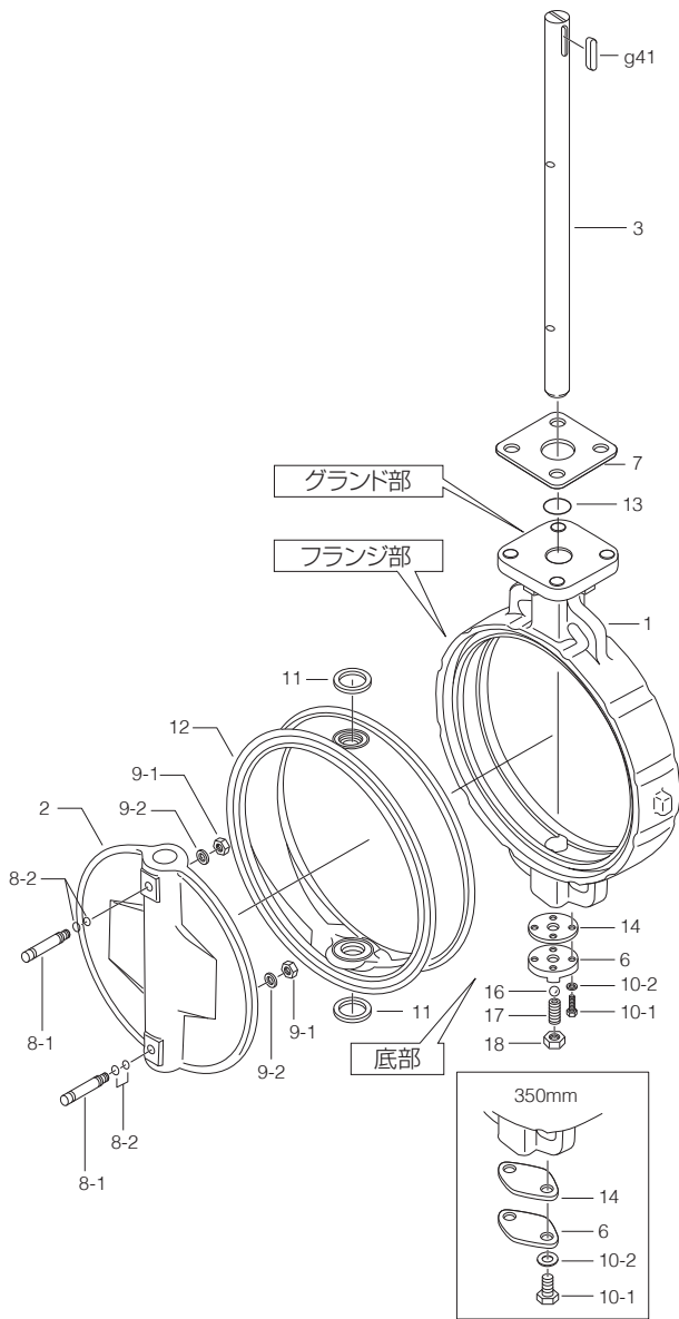
704G 350mm to 600mm
