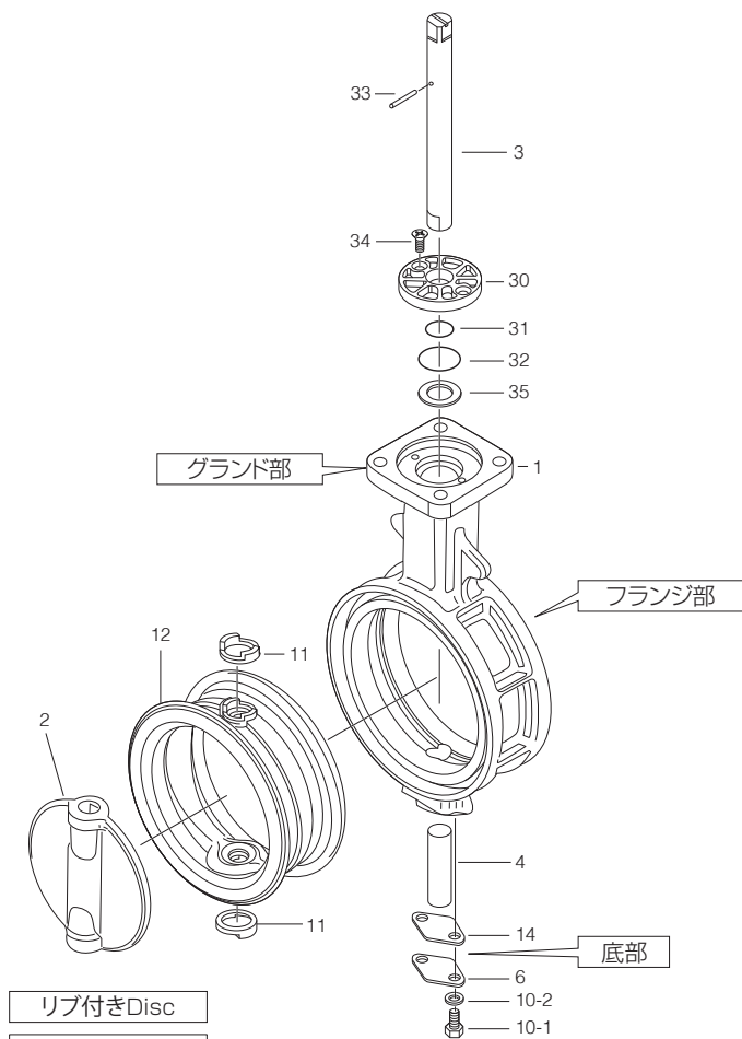
704G 80mm(JIS10K) 100mm to 300mm
