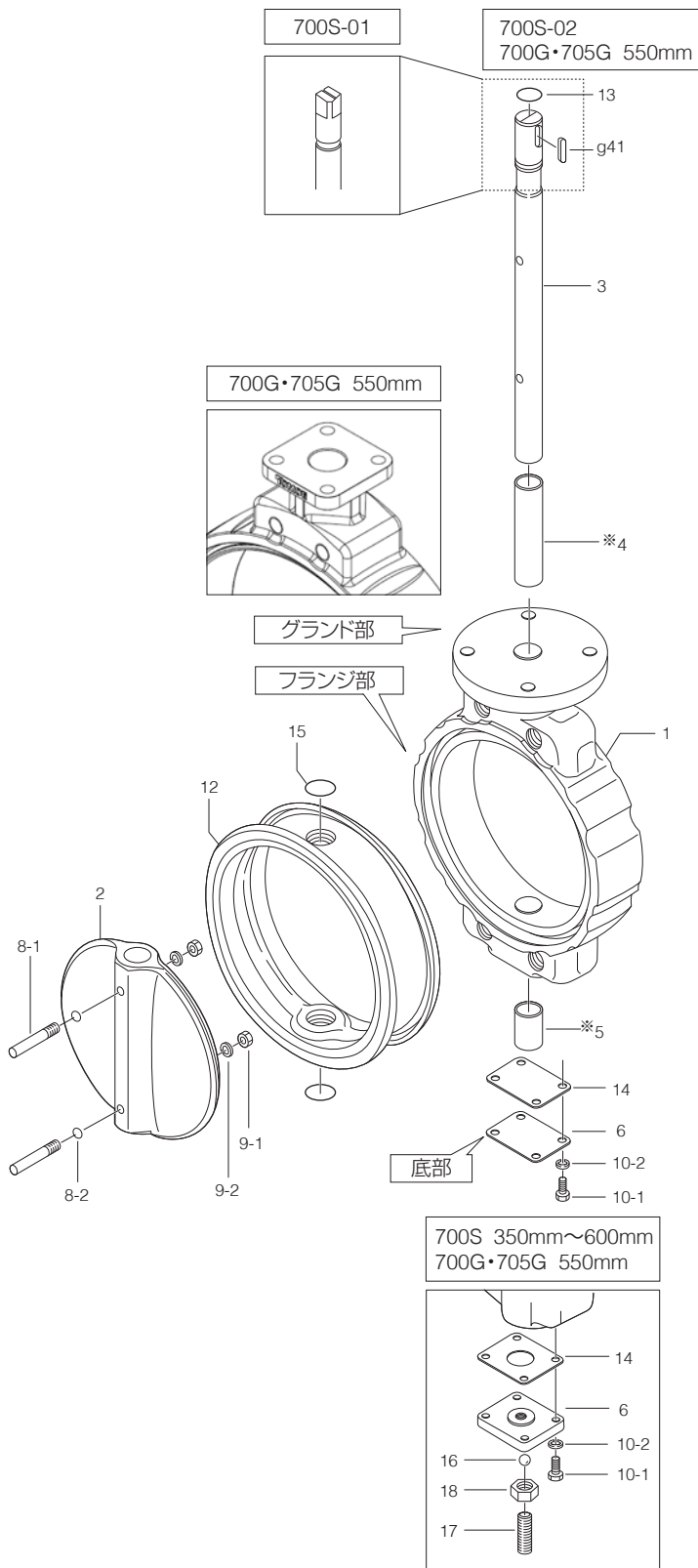
■700S本体部部品表 (700S-01/02:50mm~300mm)
