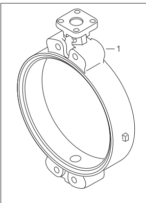
705G・731R 350mm to 600mm
